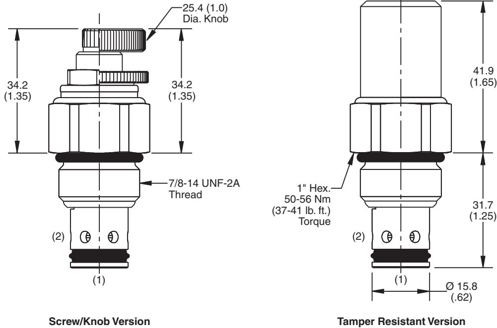
Screw/Knob Version
